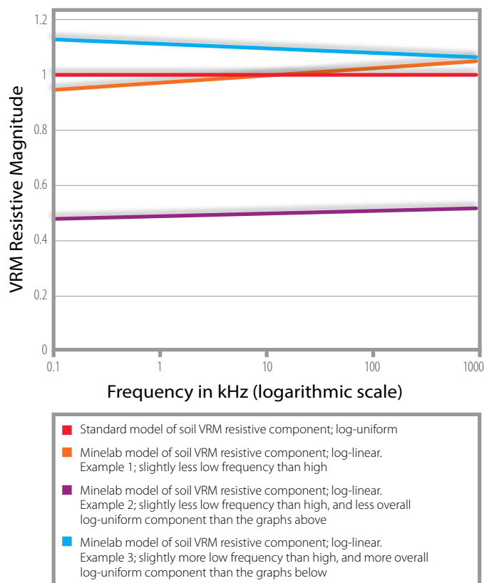
Figure 4. Different resistive VRM soils.
